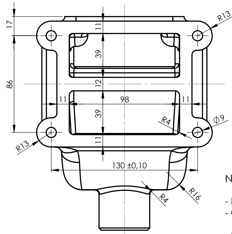
POGLED "X"
