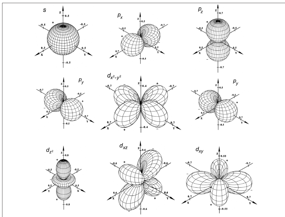
Figure 24. Angular parts (spherical harmonics) of s , p and d atomic orbitals. Drawings were handmade by using calculated coordinates of three-dimensional surfaces in normal projection.
